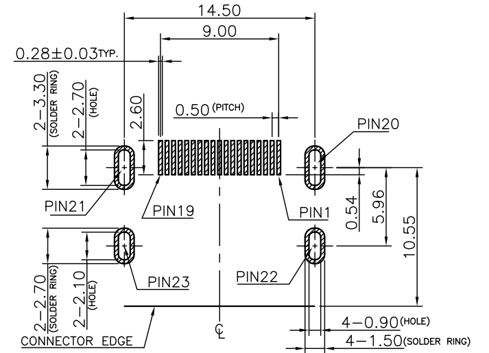
RECOMMENDED PCB LAYOUT (TOP VIEW) TOLERANCE: ±0.05mm
