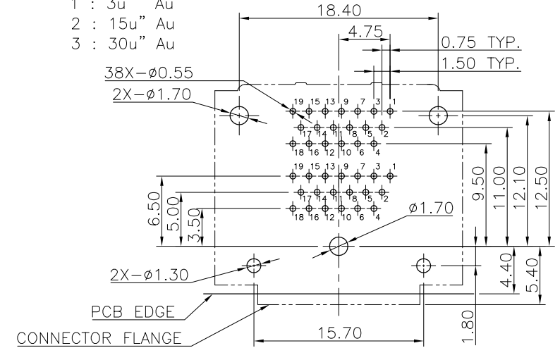
RECOMMEND PCB LAYOUT (TOP VIEW) TOLERANCE: ±0.05mm
